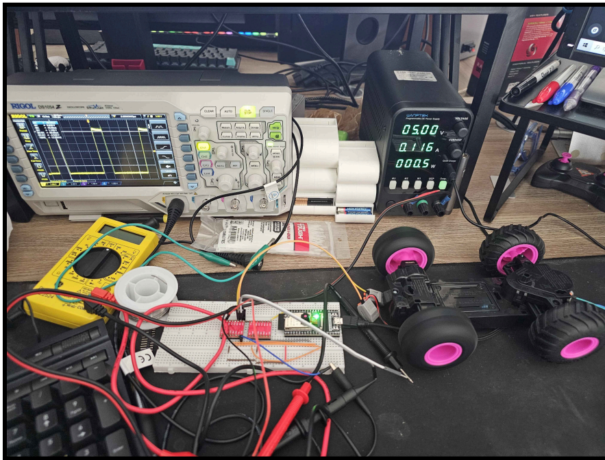
Figure 9.5. Photo from Motor Controls Tests via Motor Driver and ESP32 Connections
