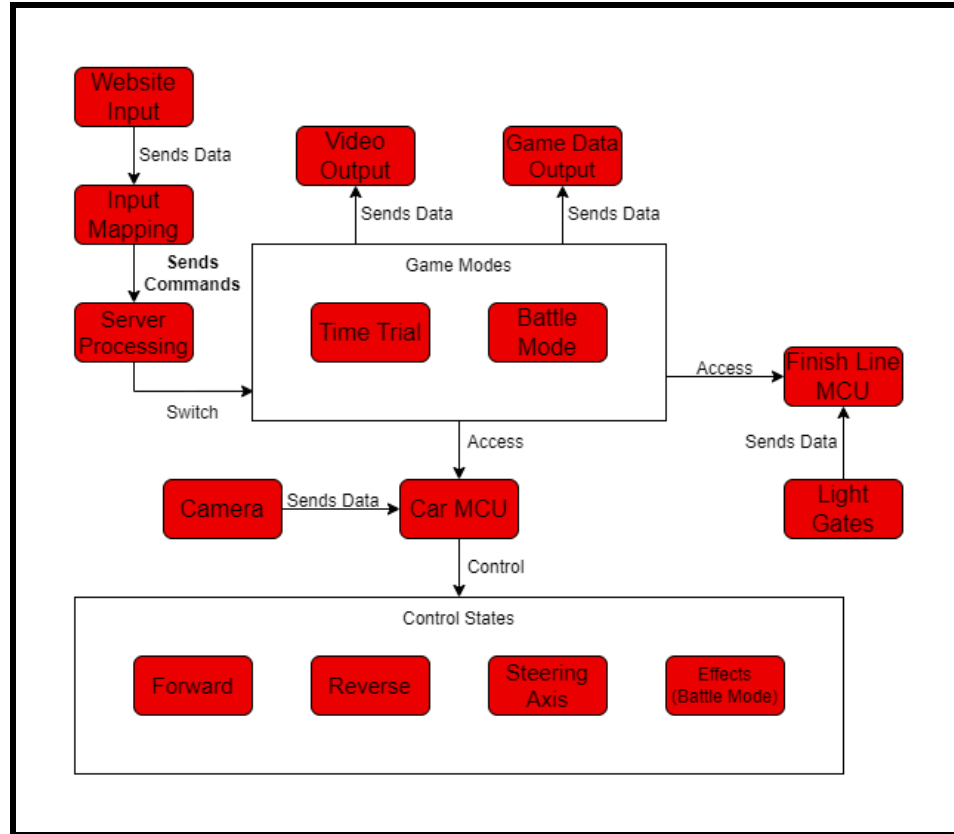
Figure 7.2. Functionality Block Diagram by Author
