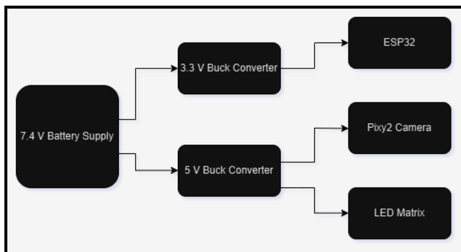
Figure 6.2. Finish Line System Power Supply Architecture
