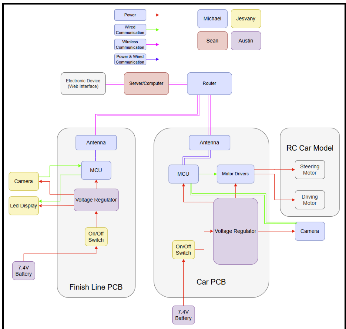
Figure 2.1. Hardware Diagram by Authors
