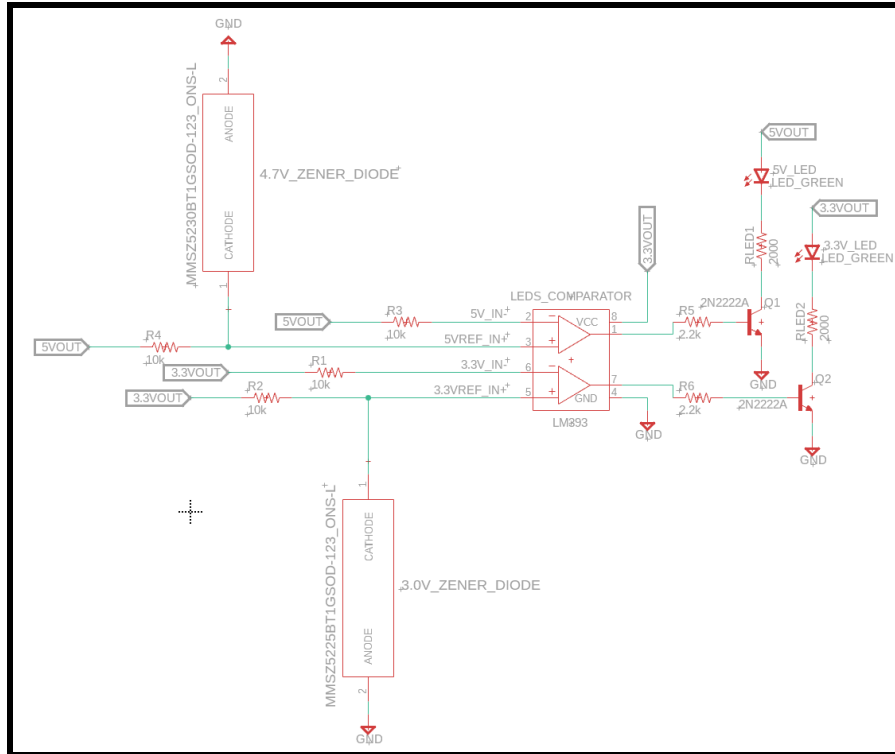
Figure 6.5. Schematic Capture of the Status LED Circuit
