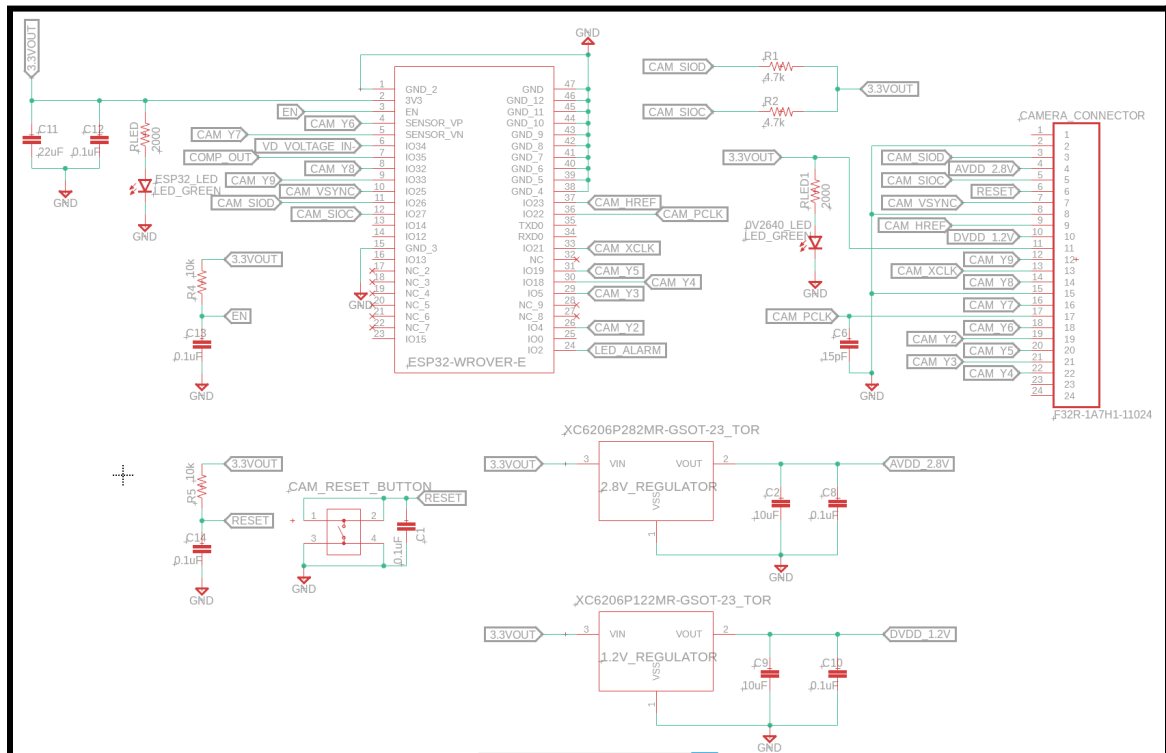
Figure 6.10. Schematic Capture of OV2640 and ESP32 Connections
