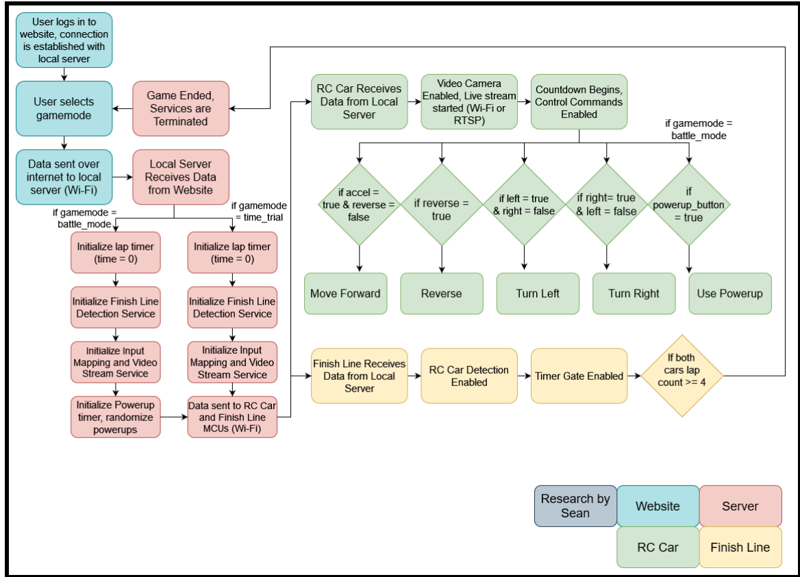
Figure 2.2. Software Flowchart by Authors
