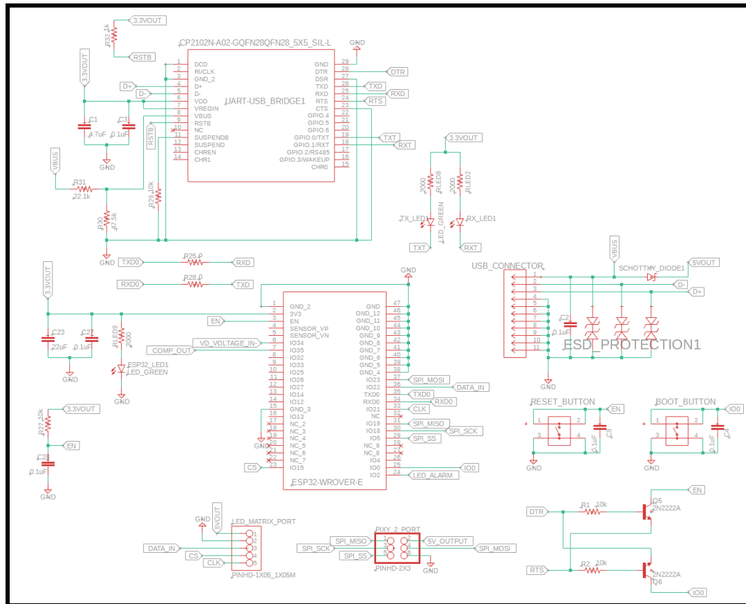
Figure 6.18. Complete Schematic of the Finish Line System
