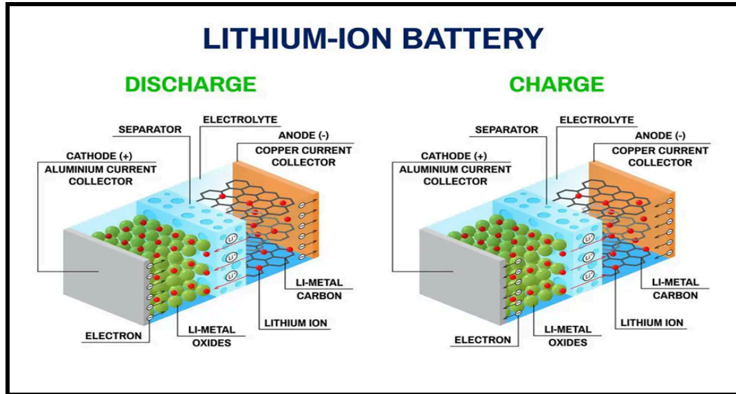
Figure 3.7. Charging and Discharging of a Lithium-Ion Battery
