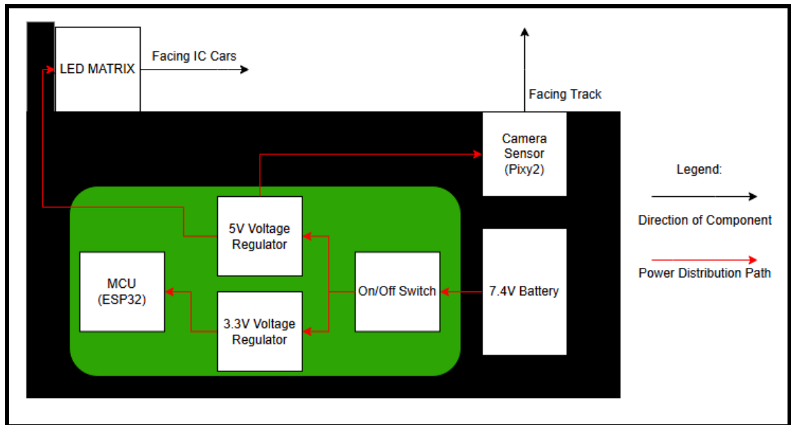
Figure 8.2. Block Diagram of Finish Line Enclosure
