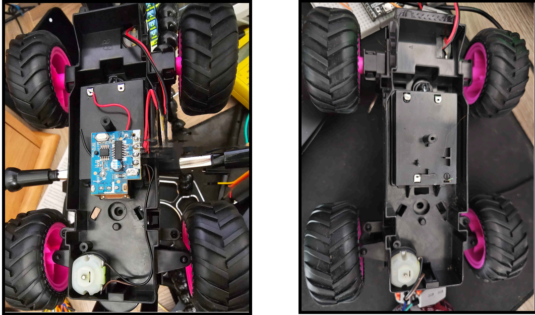
Figure 6.14. RC Car Original Setup (Left) and Removal of Parts (Right)
