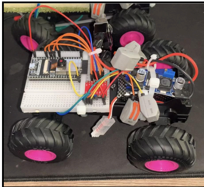
Figure 6.15. IC Car Breadboard Prototype
