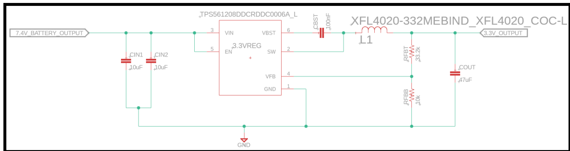
Figure 6.3. Schematic for the 3.3 V Regulator Circuit
