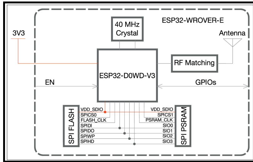
Figure 6.13. ESP32-WROVER-E Module Block Diagram
