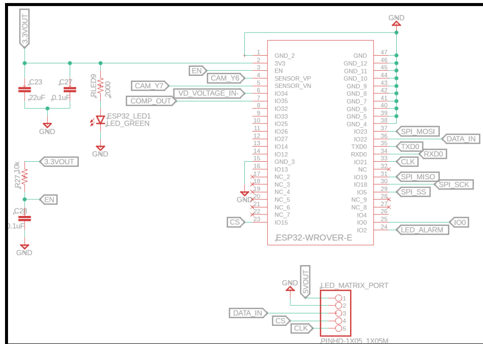
Figure 6.17. Schematic Capture of LED Matrix and ESP32 Connections
