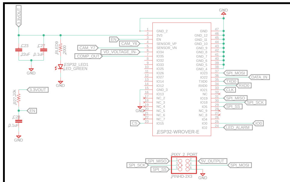
Figure 6.16. Schematic Capture of Pixy2 Camera and ESP32 Connections
