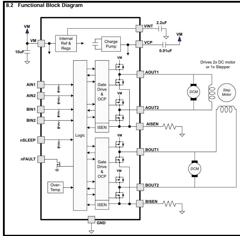
Figure 6.9. DRV8833 Functional Block Diagram via TI Datasheet
