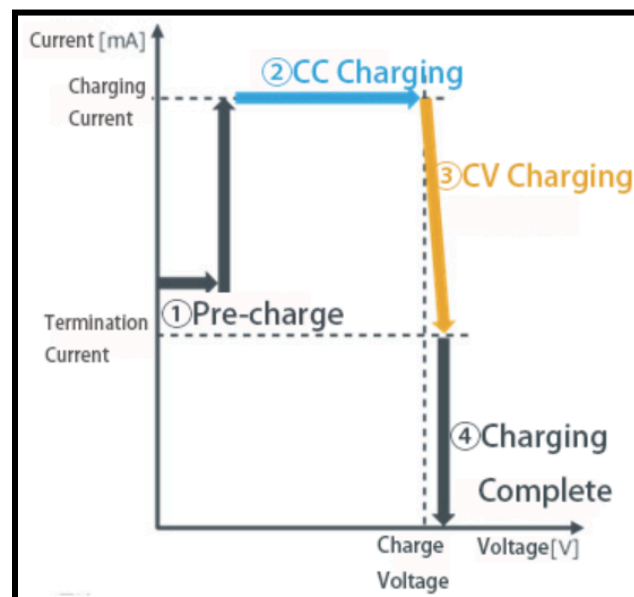
Figure 3.8. CCCV Charging Process for Li-Ion Batteries
