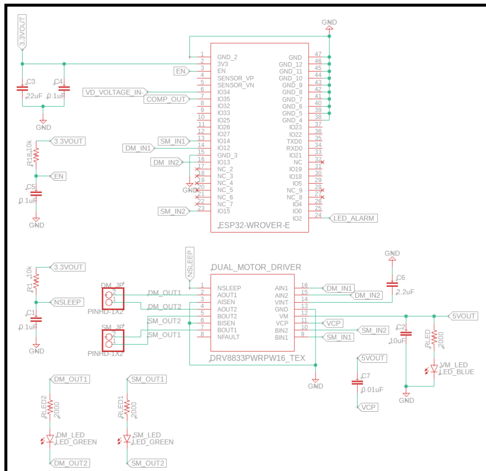
Figure 6.8. Schematic Capture of Motor Driver and ESP32 Connections
