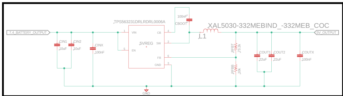
Figure 6.4. Schematic for the 5 V Regulator Circuit
